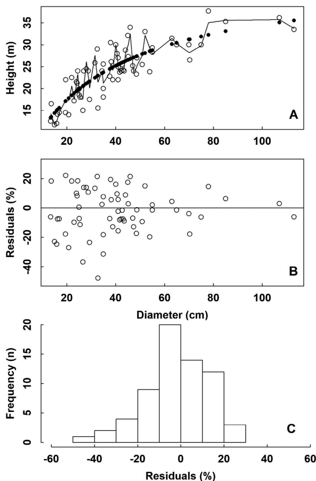
Figure 2. Best-performing allometric model (Michaelis-Menten) fitted to predict total height from stem diameter for trees in an ecotone zone of northern Brazilian Amazonia. Where: A = observed values (empty circles), estimated values (black circles) and black line (smoothed fit, 10%), B = dispersion of residuals (%), C = distribution of frequencies of occurrence of residuals (n).
